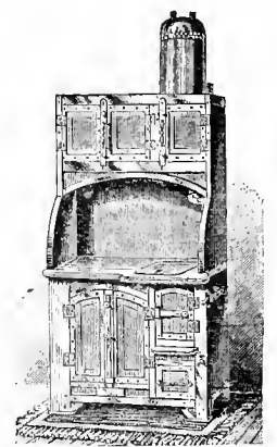
Fig. 3108. DIRECTORS'-CAR RANGE, with hot-water tank. Size, 2 ft. 6 in. x 1 ft. 10 in. x 5 ft. 0 in. Weight, 490 lbs.
